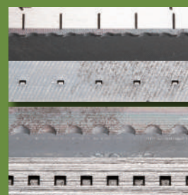
Custom-jaws tooth profile samples
